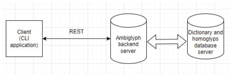
Fig. 8 Client-server structure
