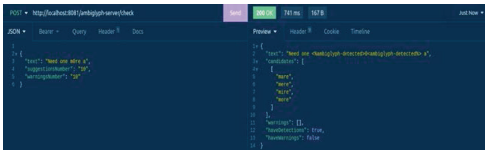
Fig. 10 Obfuscated word “more” (“m0re”) is detected, and suggestions are provided.
