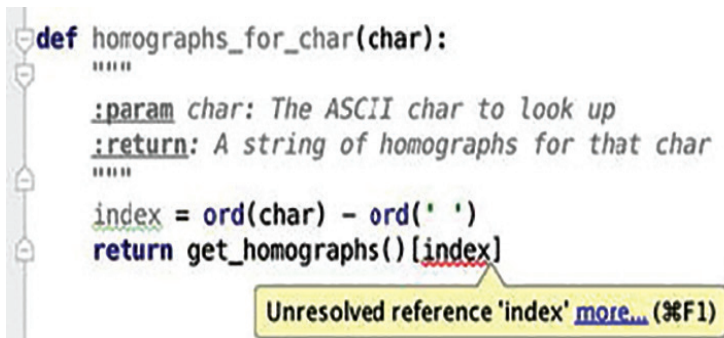
Fig. 4 Static analyzer inside IDE recognizes spoofed variable as a new uninitialized variable. ( https://habr.com/ru/post/385697 )
