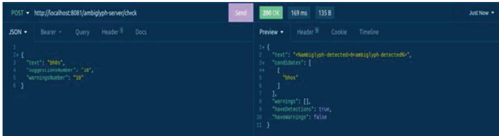
Fig. 13 Word “bh0s” recognized as obfuscated word “bhos.”
